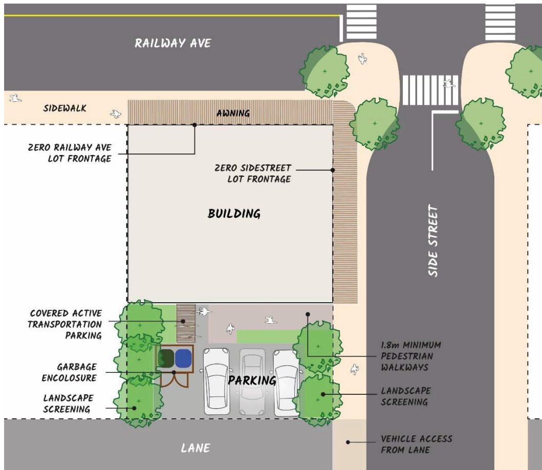
Figure G 3: Example Site Design
